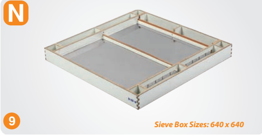
N N Tipi Kasa N Type Sieve Box
